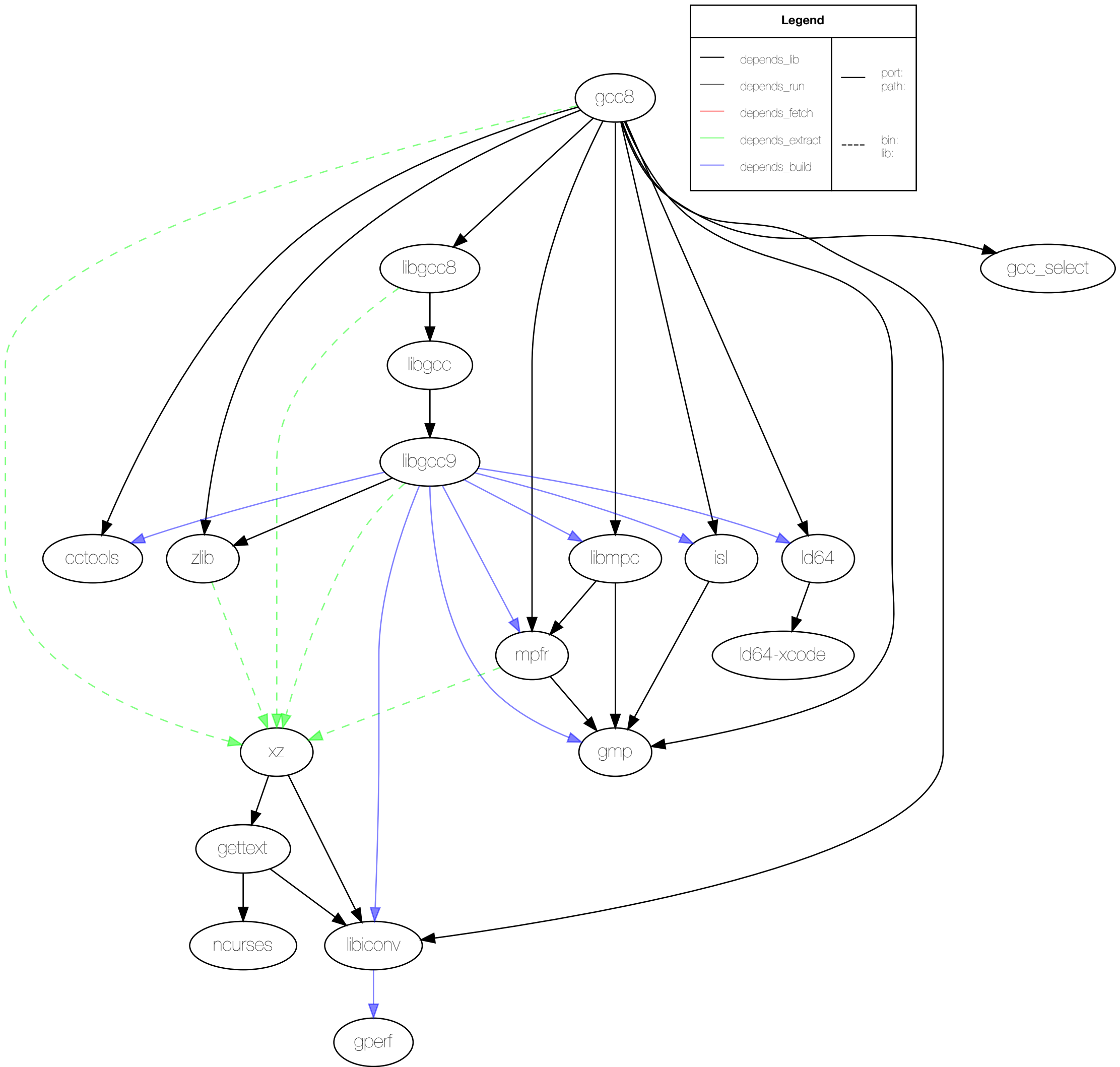
Dependencies of gcc8 +xcode
